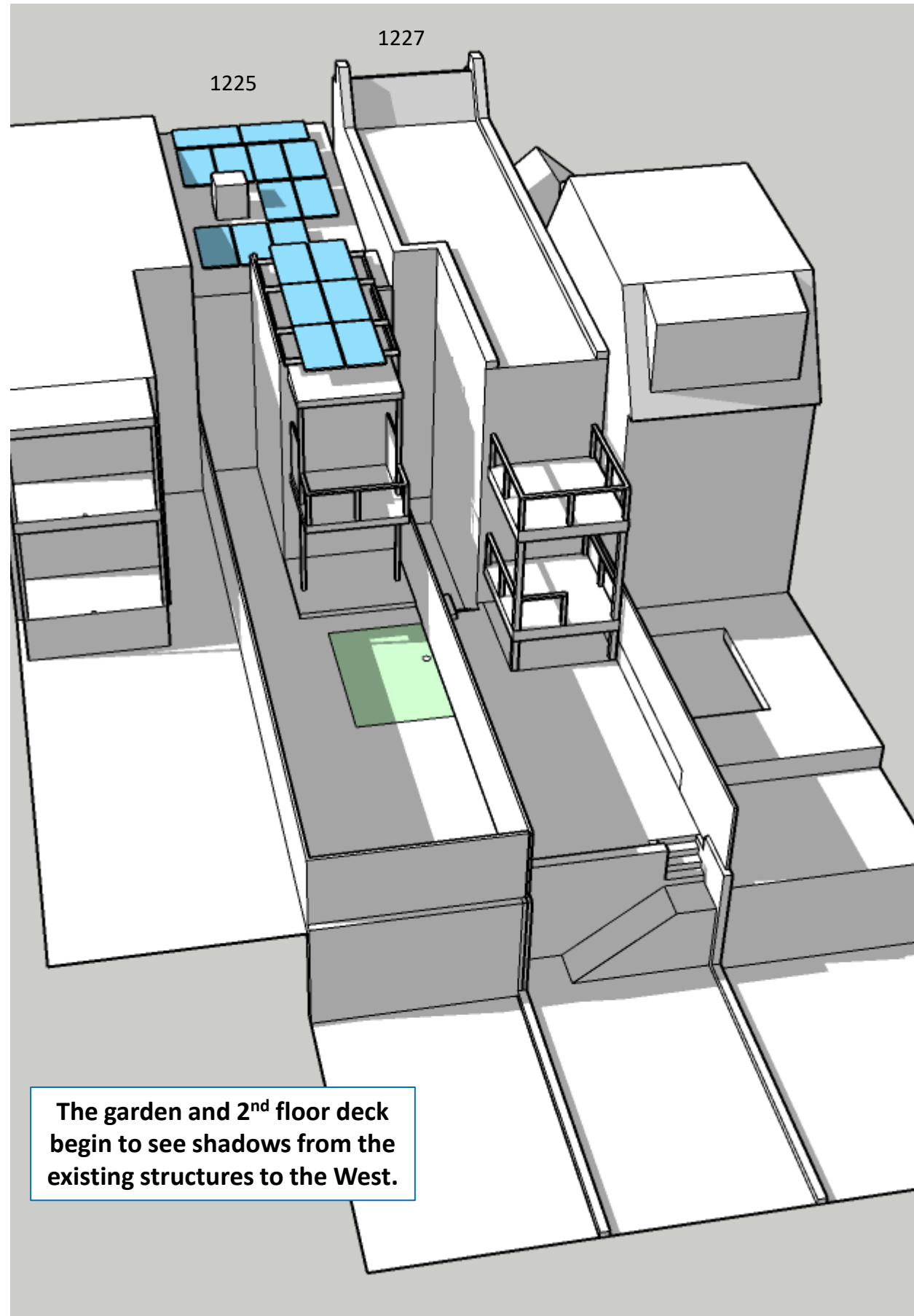
Existing Conditions – 4:30pm June 21
