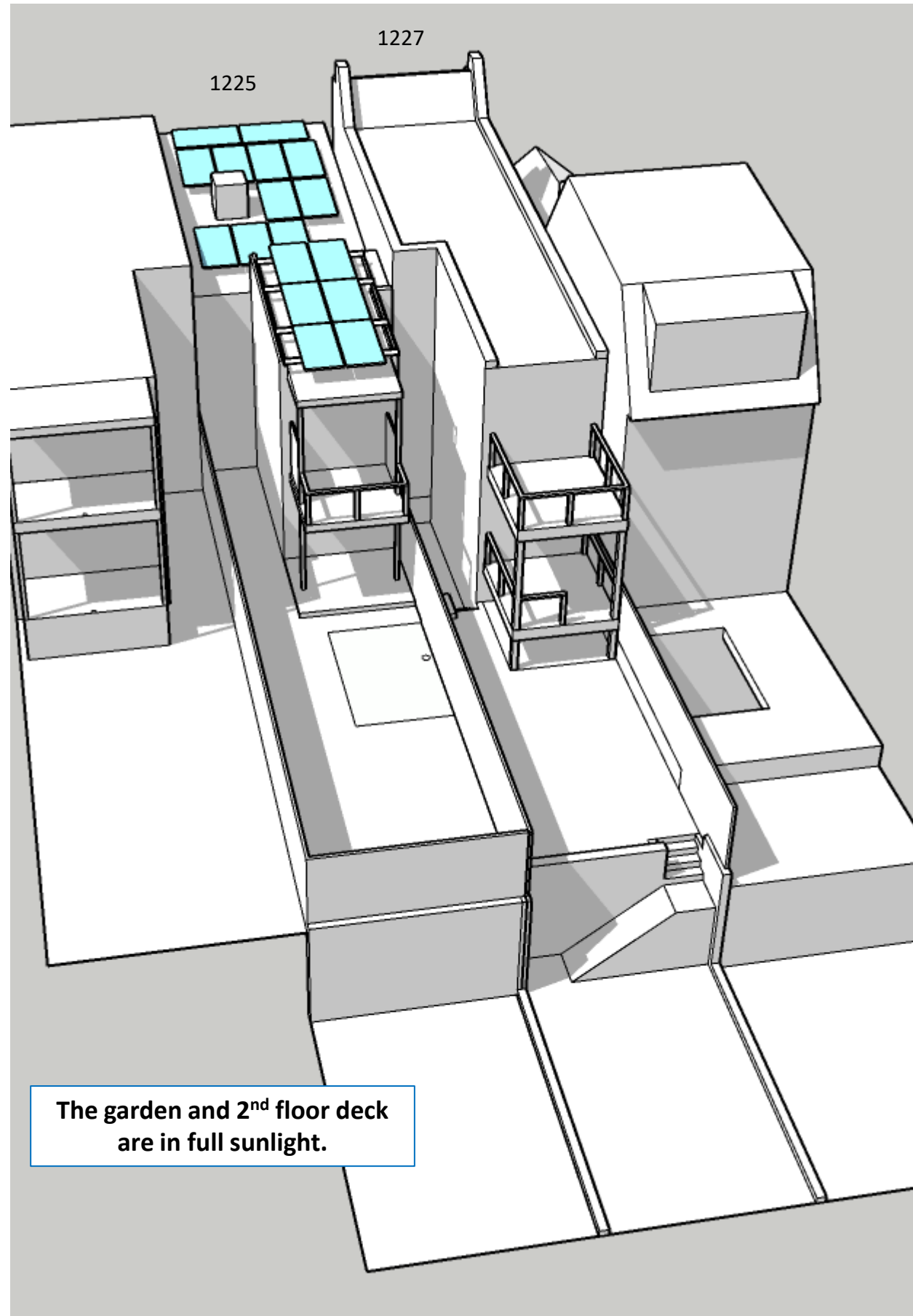
Existing Conditions – 2:30pm June 21
