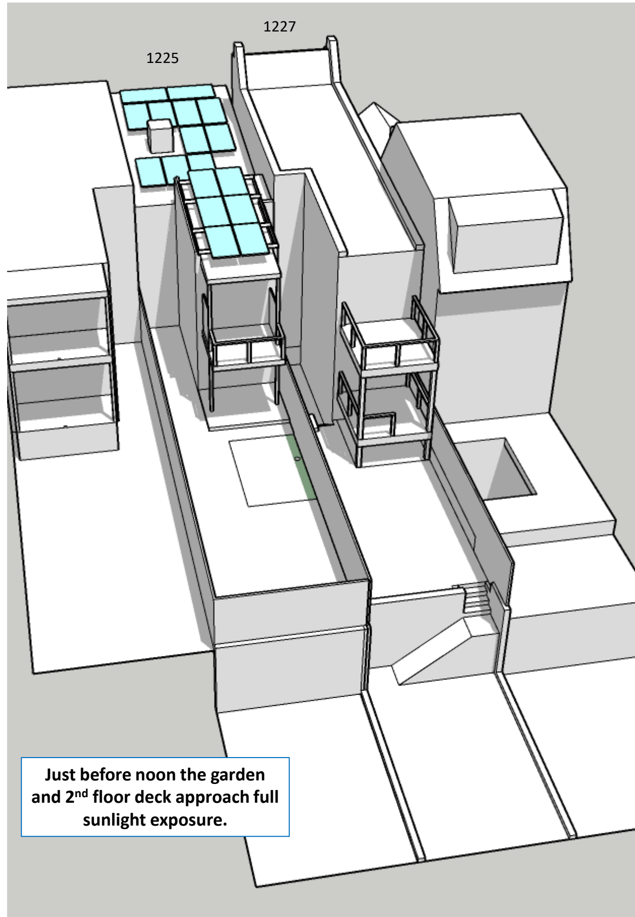
Existing Conditions – 11:30am June 21
