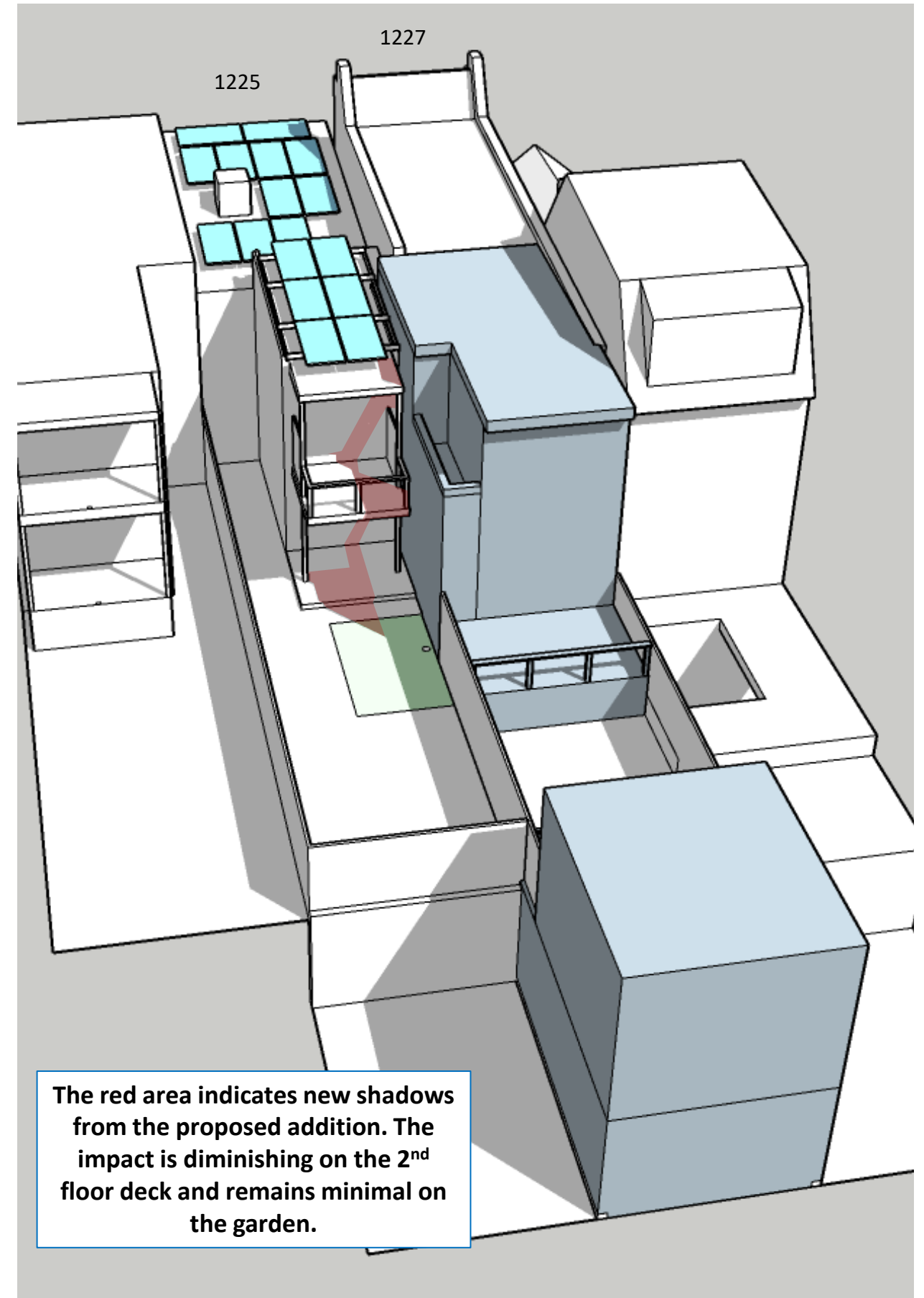
Proposed Addition – 10:30am April 7
