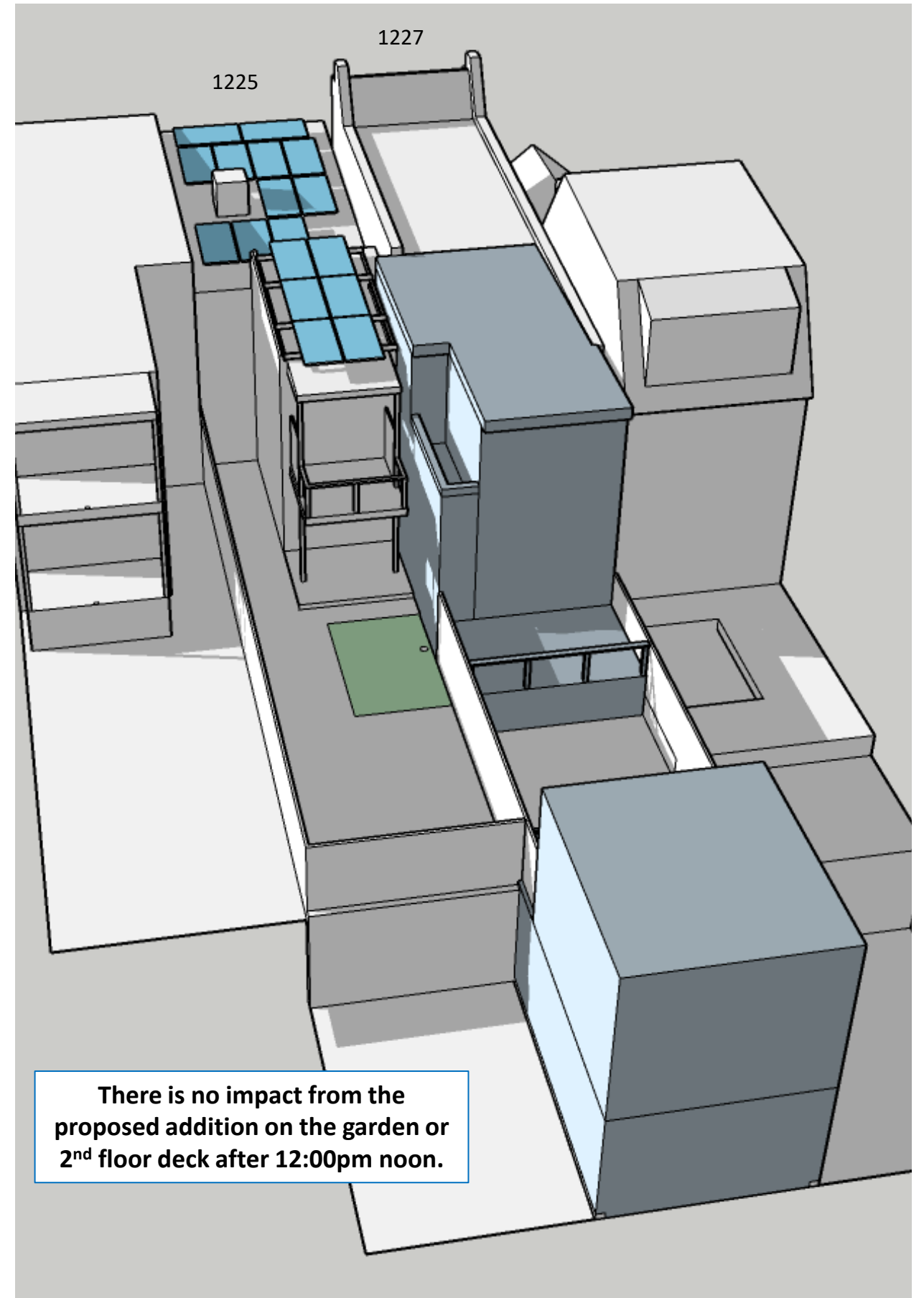
Proposed Addition – 5:30pm June 21
