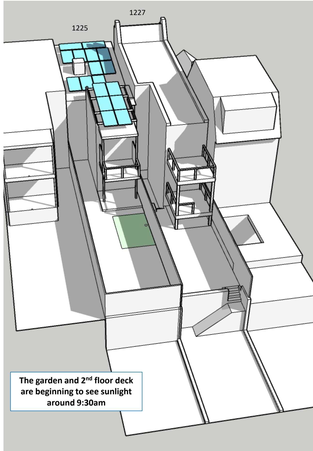
Existing Conditions – 9:30am April 7
