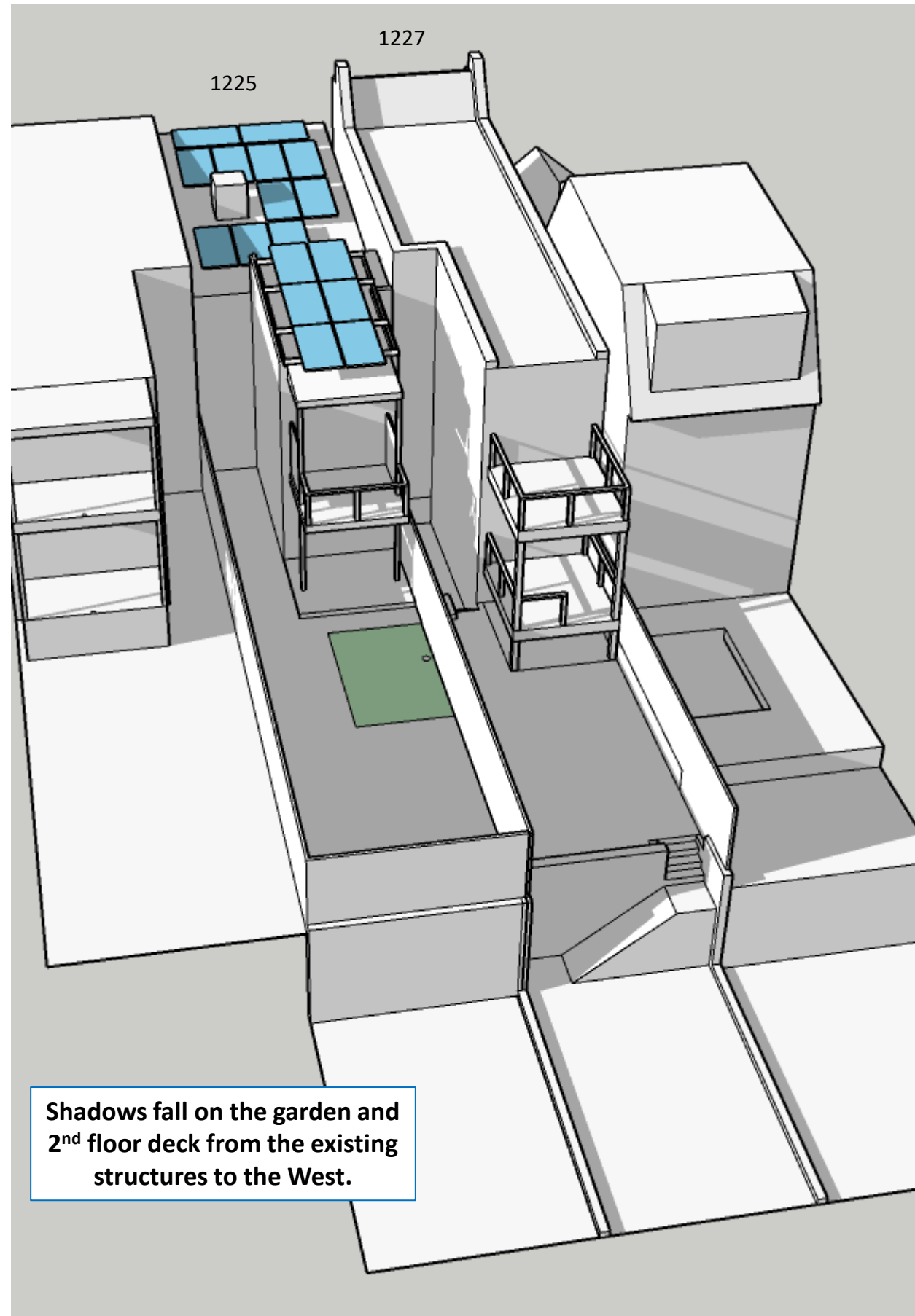
Existing Conditions – 4:30pm April 7
